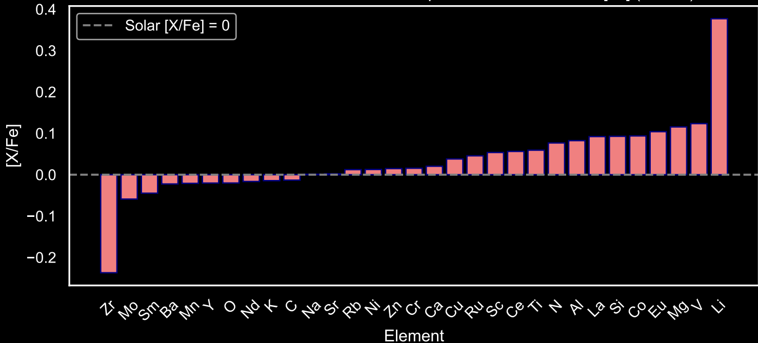
Abundance Pattern for GALAH Main Sequence Stars: Star Field [47] (N=142)
