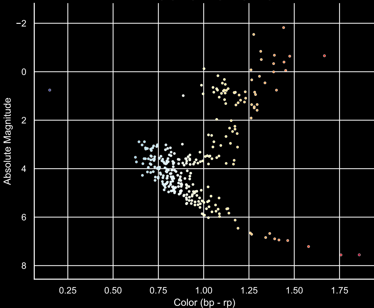
GALAH Hertzprung-Russel Diagram Field [47] Ra [322.94] Dec [-54.13]
