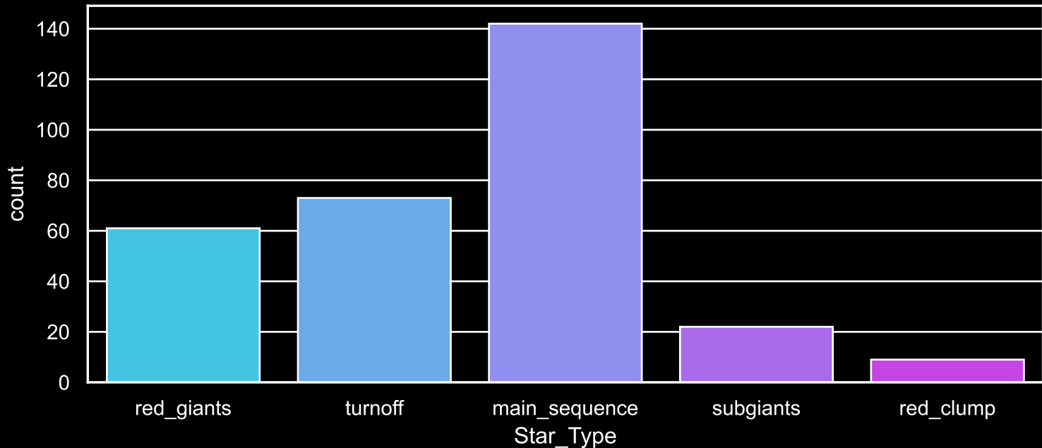
Field [47] Count plot of Star Type
