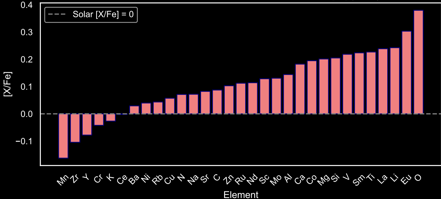
Abundance Pattern for GALAH Red Giants: Star Field [47] (N=70)
