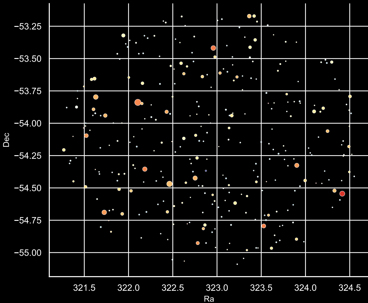
Field [47] Ra [322.94] Dec [-54.13] Stars: 307
