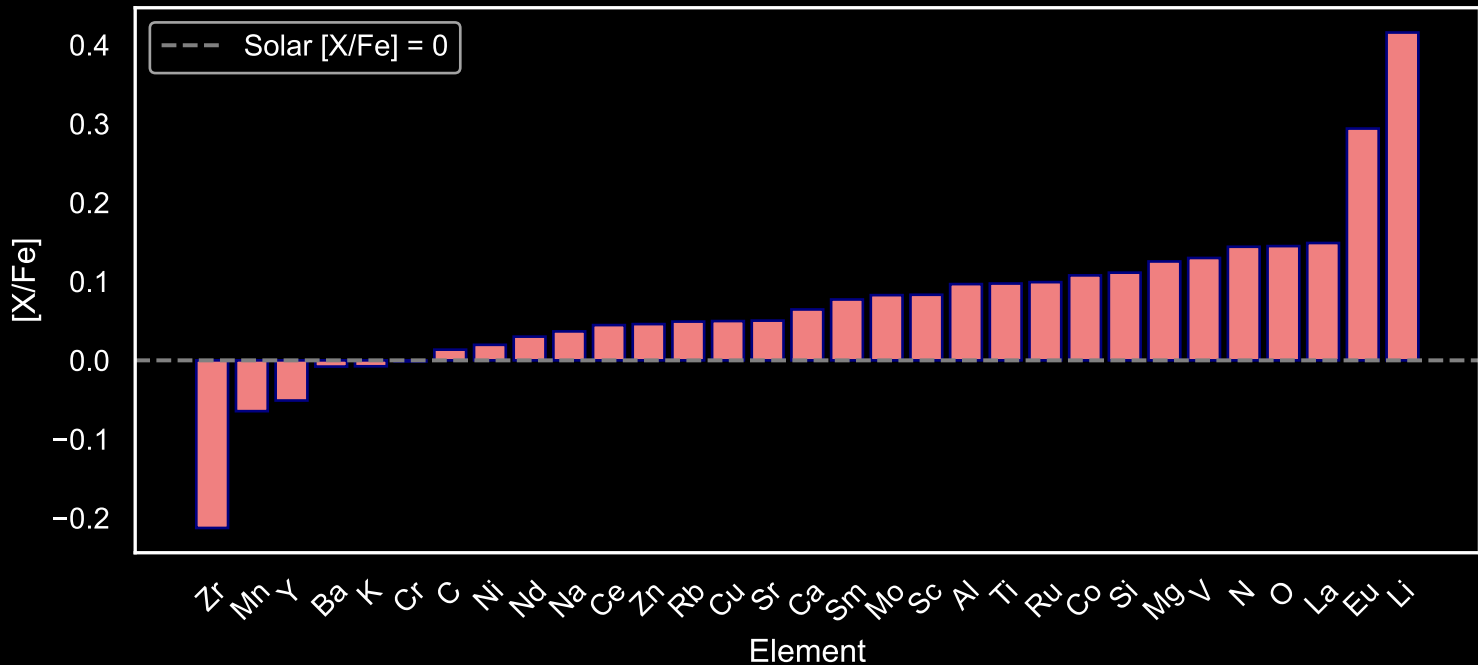
Abundance Pattern for GALAH Star Field [47] (N=307)
